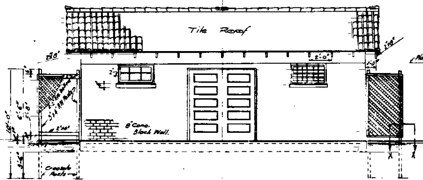
SIDE ELEVATION Scale 1/2" = 1'
