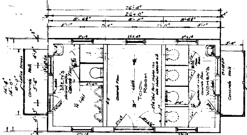
PLAN Scale 1/2" = 1'
