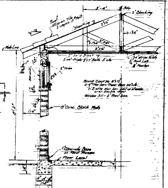
PART SECTION Scale 1/2" = 1'
