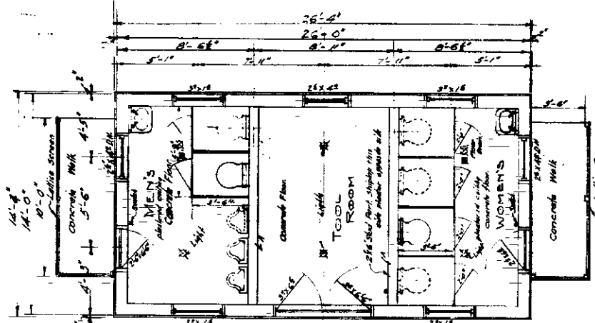
PLAN Scale 1/2" = 1'
